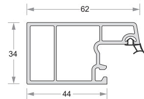
Casement Indiana Sash/style DP34-IN-353
