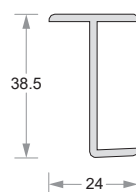
Casement Indiana "T" Profile DP34-IN-362
