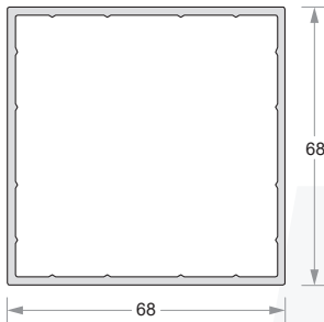
Square Bay Pole DP-UN-328
