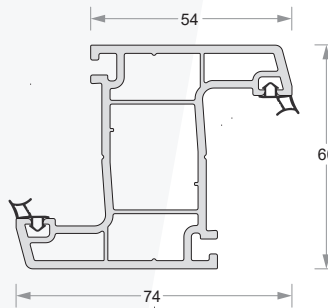
Casement 'Z' Mullion DP60-EL-658
