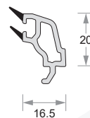
Glazing Bead (24mm) DP60-EL-661
