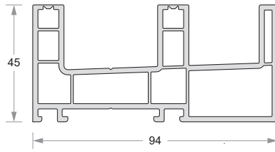
Sliding 2 Track Frame With Mesh Rail DP60-EL-602
