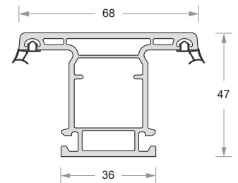
Sliding Sash Mullion DP67-ET-713
