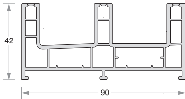
Sliding 3 Track Frame DP50-EG-503-01
