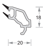
Glazing Bead (5mm) DP60-EL-614
