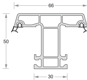
Casement Transom/Mullion DP50-EG-557
