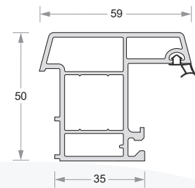
Casement Fly Mullion DP50-EG-559
