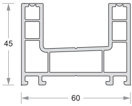
Sliding 2 Track Frame DP60-EL-601
