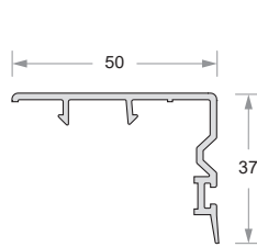
Sliding Window Interlock DP67-ET-709
