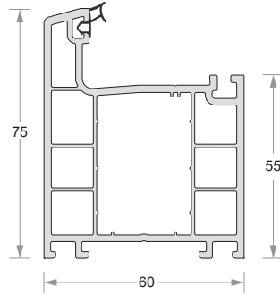
Casement Frame - Large DP60-EL-652
