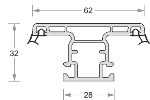
Sliding Sash Mullion DP50-EG-513
