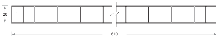
Single Panel DP-SS-610
