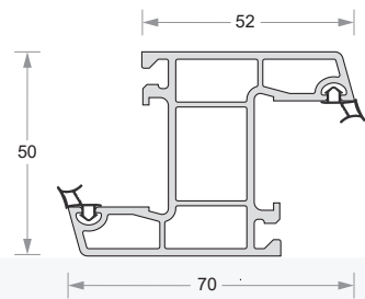
Casement "Z" Mullion DP50-EG-558
