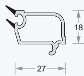
Glazing Bead (5mm) DP50-EG-560
