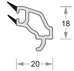
Glazing Bead (5mm) DP60-EL-614
