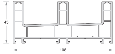
Sliding 3 Track Frame DP60-EL-603
