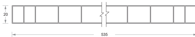
Single Panel DP-SS-535
