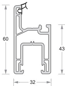
Sliding Window Sash DP50-EG-506
