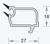
Glazing Bead (20mm) DP50-EG-560
