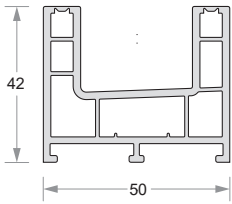
Sliding 2 Track Frame DP50-EG-501-01
