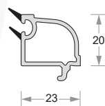
Glazing Bead (24mm) DP67-ET-761
