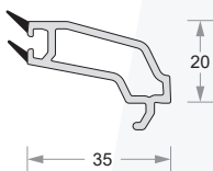
Glazing Bead (5mm) DP60-EL-660
