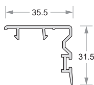
Sliding Window Interlock DP50-EG-509
