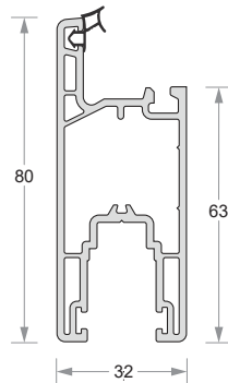
Sliding Flexi Sash DP50-EG-508
