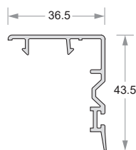
Sliding Flexi Interlock DP50-EG-511
