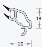
Glazing Bead (20mm) DP60-EL-614
