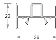
Inline Sash Adaptor DP50-EG-520
